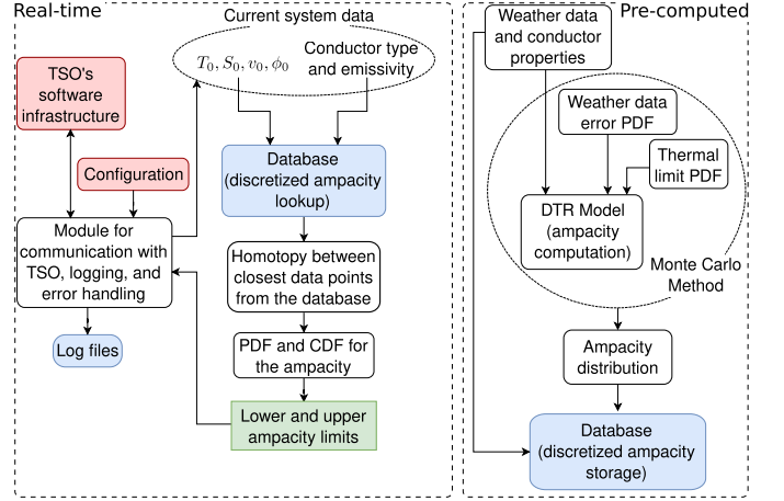
Fig. 10. Schematic representation of the operative DTR uncertainty estimation.
