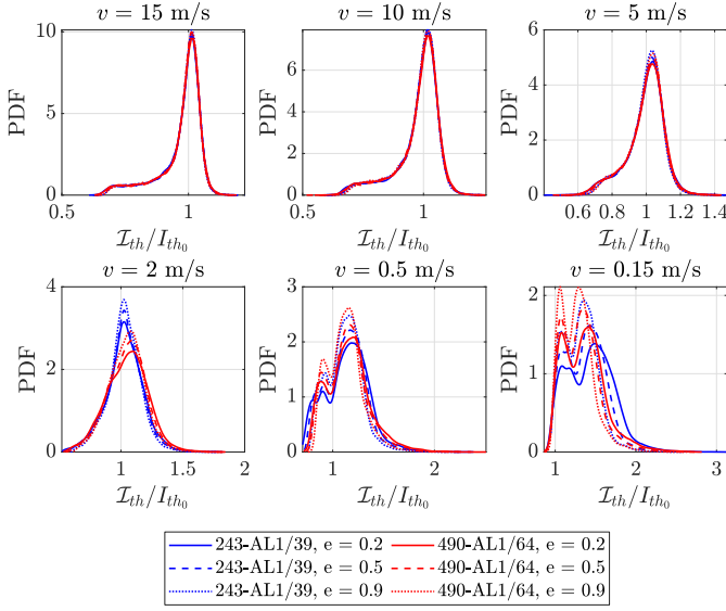
Fig. 8. Normalized ampacity distributions for two conductor types and three values of emissivity: 0.2, 0.5 and 0.9, and for different values of predicted wind speed. The values for the other parameters are: ambient temperature 15 °C, solar irradiance 500 W/m 2 , and wind direction 90°.
