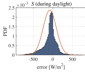
Fig. 2. Error distribution for the solar irradiance, omitting the zero values, compared to normal distribution (red curve), for Bevkov vrh.
