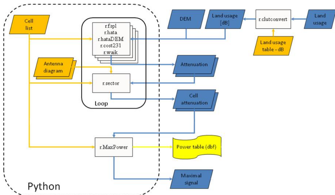
Fig. 1: GRASS-RaPlaT block diagram
