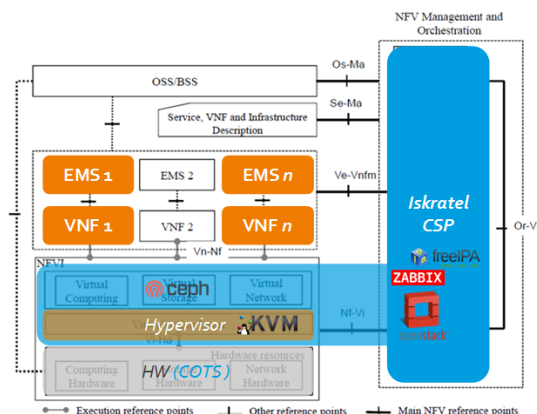
Figure 3: CSP in NFV Architecture
